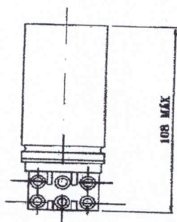
VISTA FRONTAL
